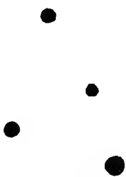
THE "SOUTHERN CROSS" AS IT ONCE WAS
